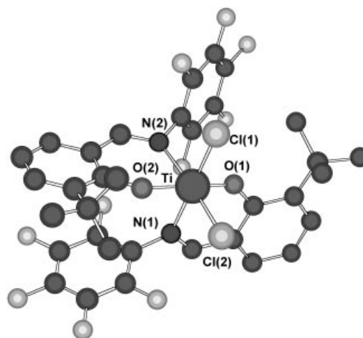
Figure 1. X-ray structure of 1 . Hydrogen atoms and a \text{CH}_2\text{Cl}_2 molecule have been omitted for clarity. Selected bond lengths [Å] and angles [°]: Ti-O(1) 1.841(3), Ti-O(2) 1.841(3), Ti-N(1) 2.240(4), Ti-N(2) 2.219(4), Ti-Cl(1) 2.289(2), Ti-Cl(2) 2.261(2); O(1)-Ti-O(2) 163.6(1), N(1)-Ti-N(2) 87.2(1) Cl(1)-Ti-Cl(2) 96.42(6).
